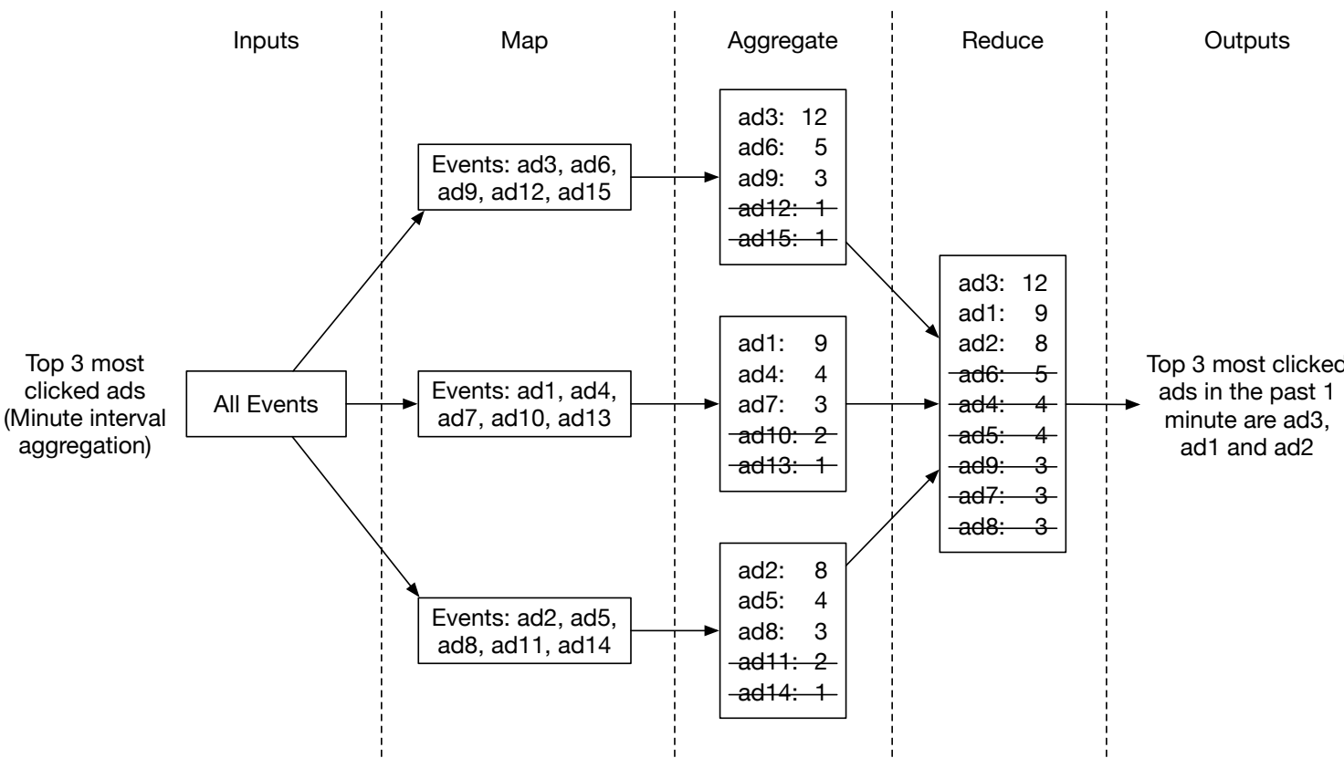
Figure 9 Return top N most clicked ads
