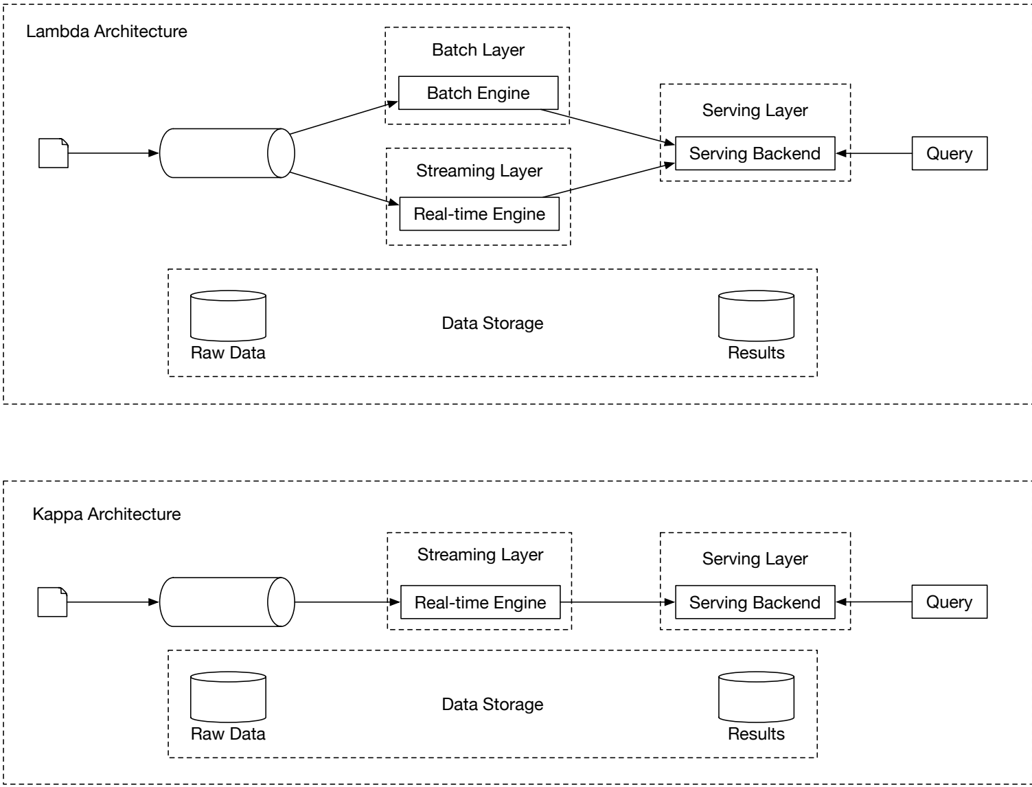
Figure 10 Lambda and Kappa architectures
