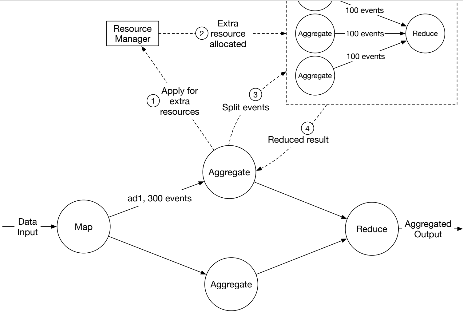
Figure 25 Allocate more aggregation nodes
