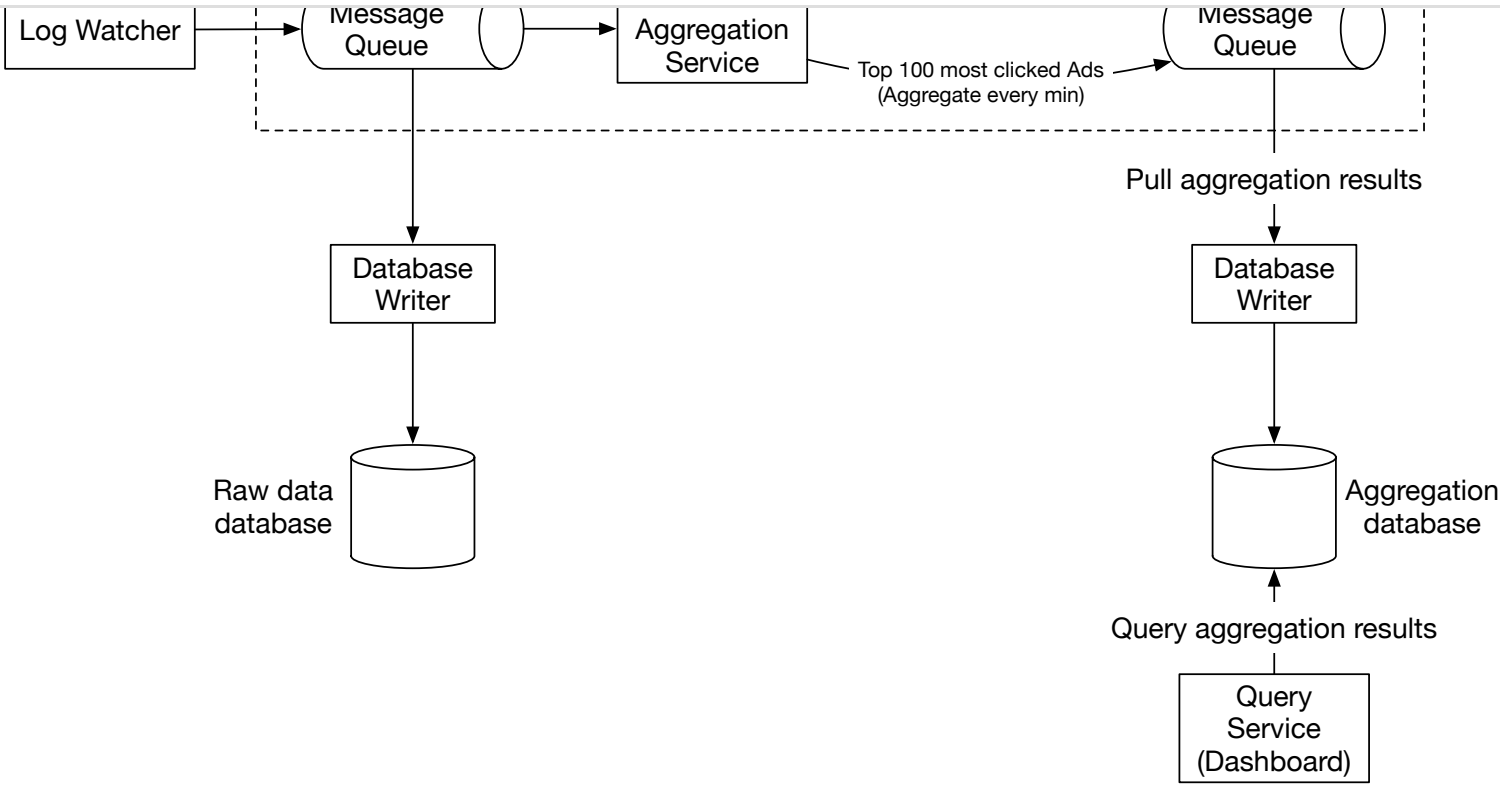
Figure 4: End-to-end exactly once
