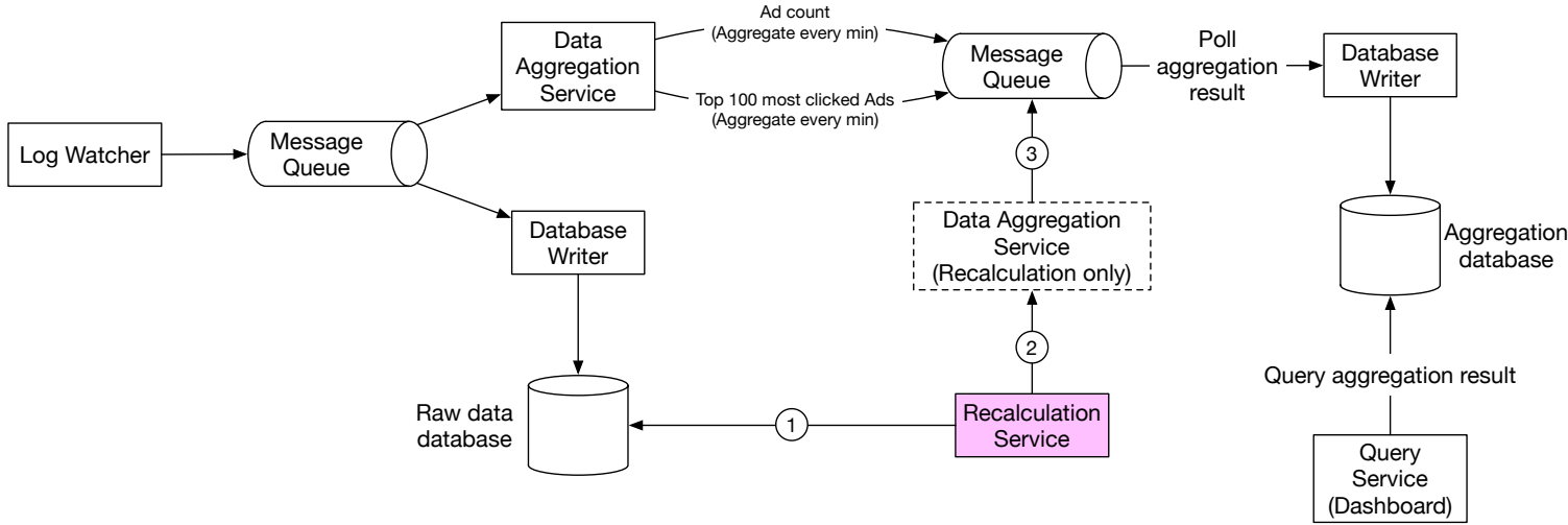
Figure 11 Recalculation service
