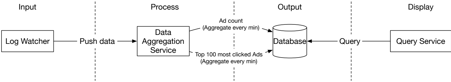
Figure 2 Aggregation workflow
