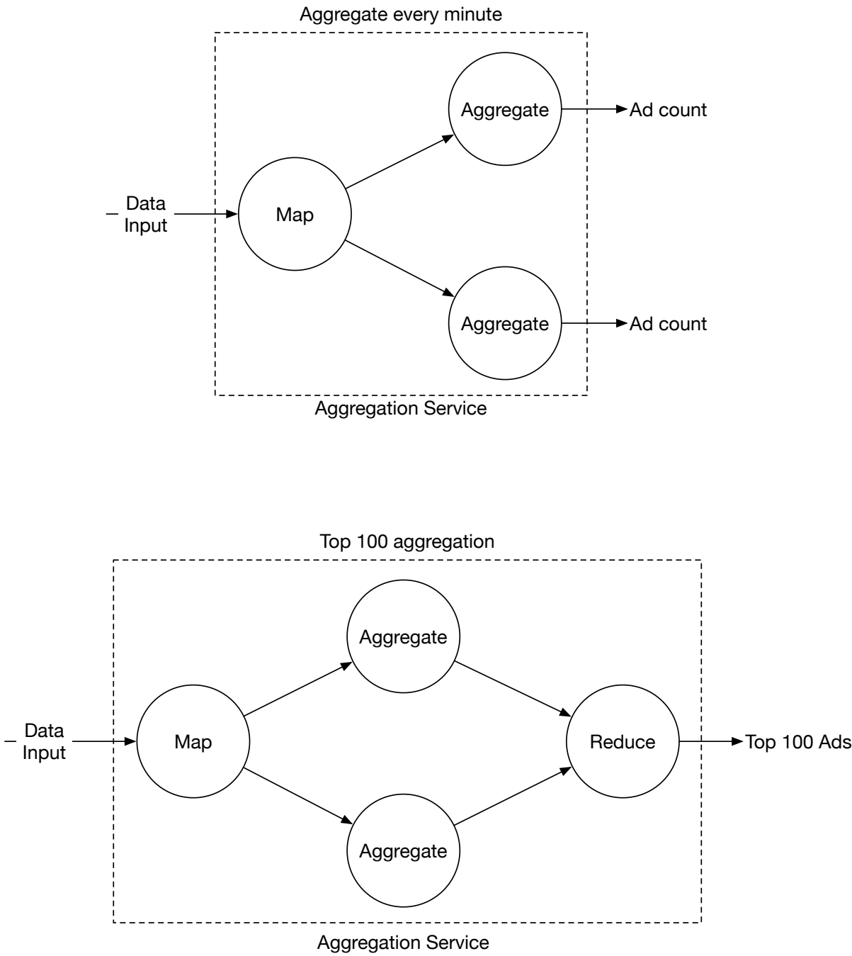
Figure 5 Aggregation service
