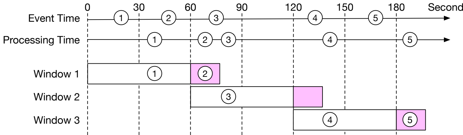
Figure 14 Watermark
