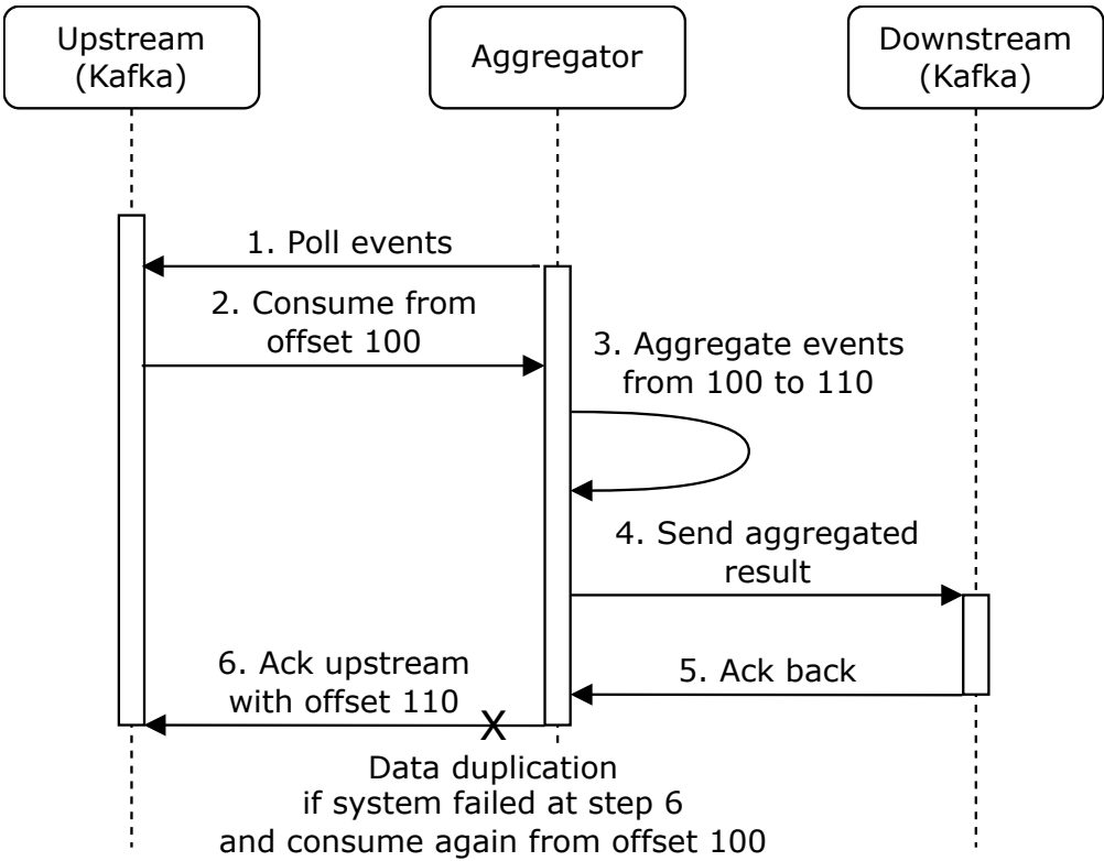
Figure 17 Duplicate data
