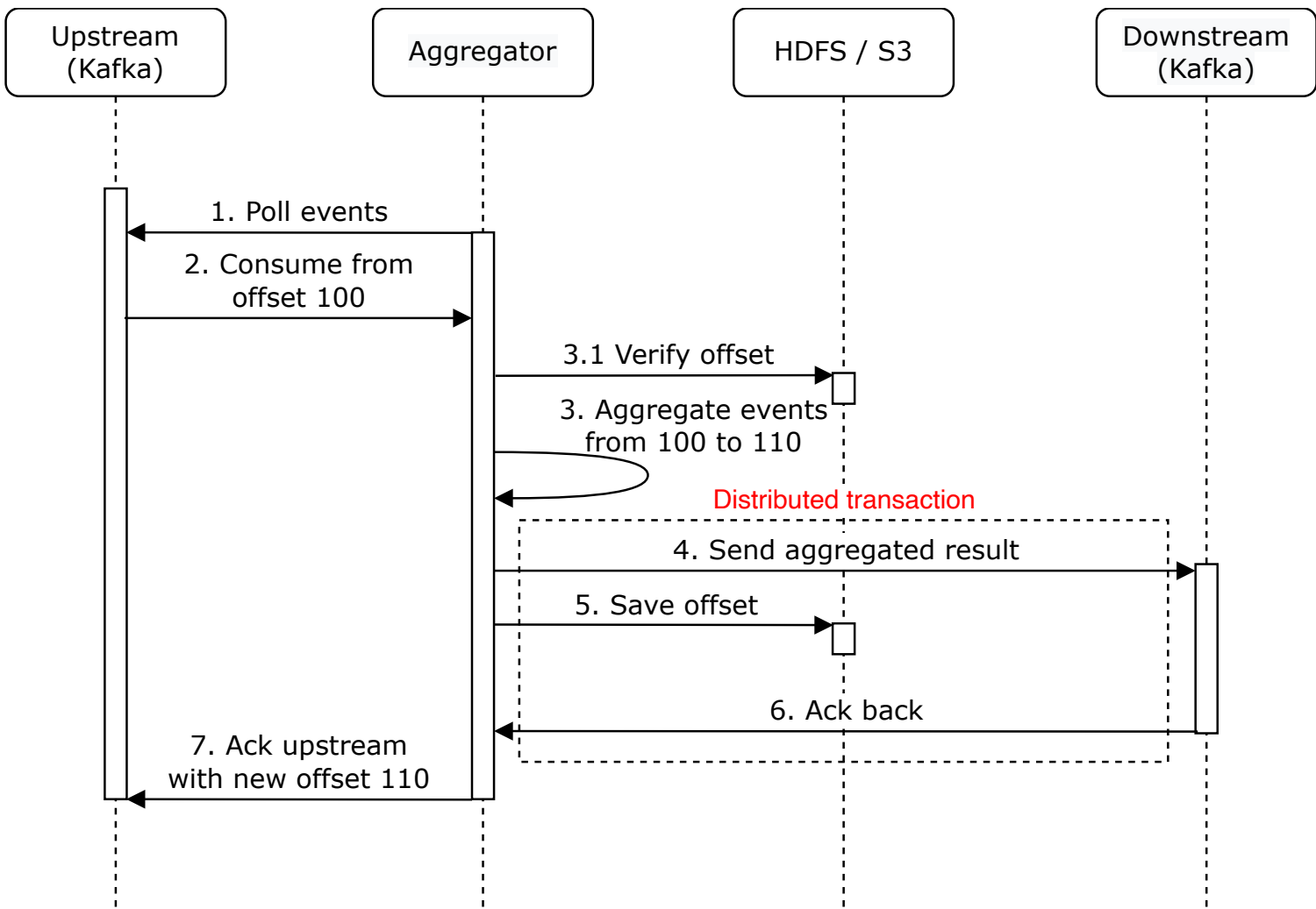
Figure 20 Distributed transaction
