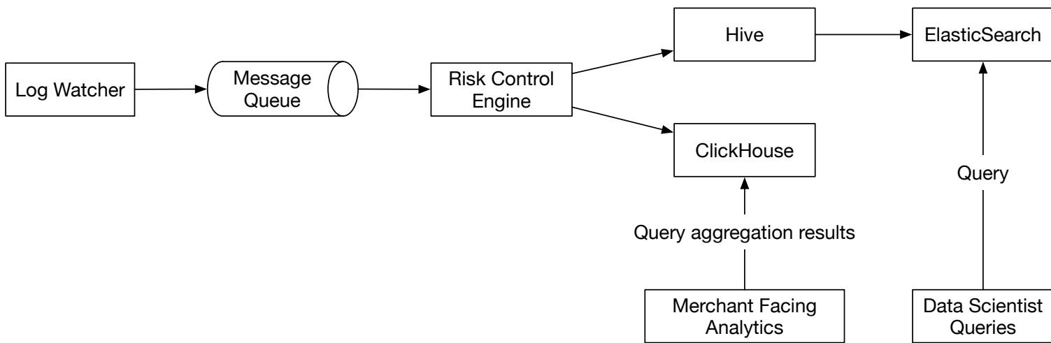
Figure 29 Alternative design
