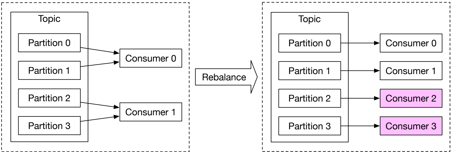
Figure 21 Add consumers
