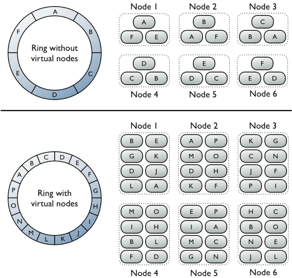
Figure 24 Virtual nodes [22]
