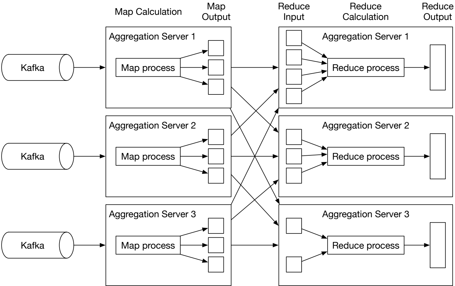
Figure 22 Aggregation service
