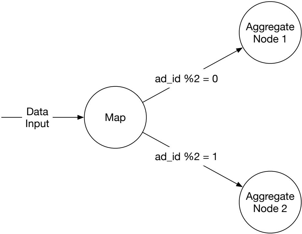
Figure 6 Map operation
