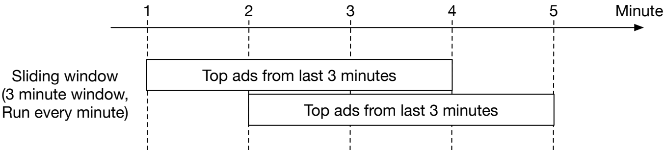
Figure 16 Sliding window
