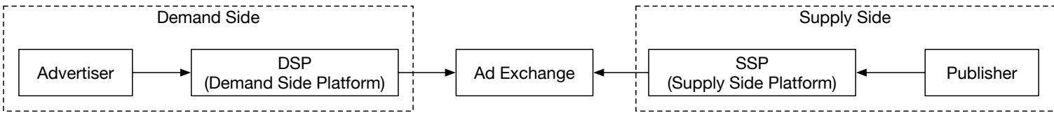
Figure 1 RTB process
