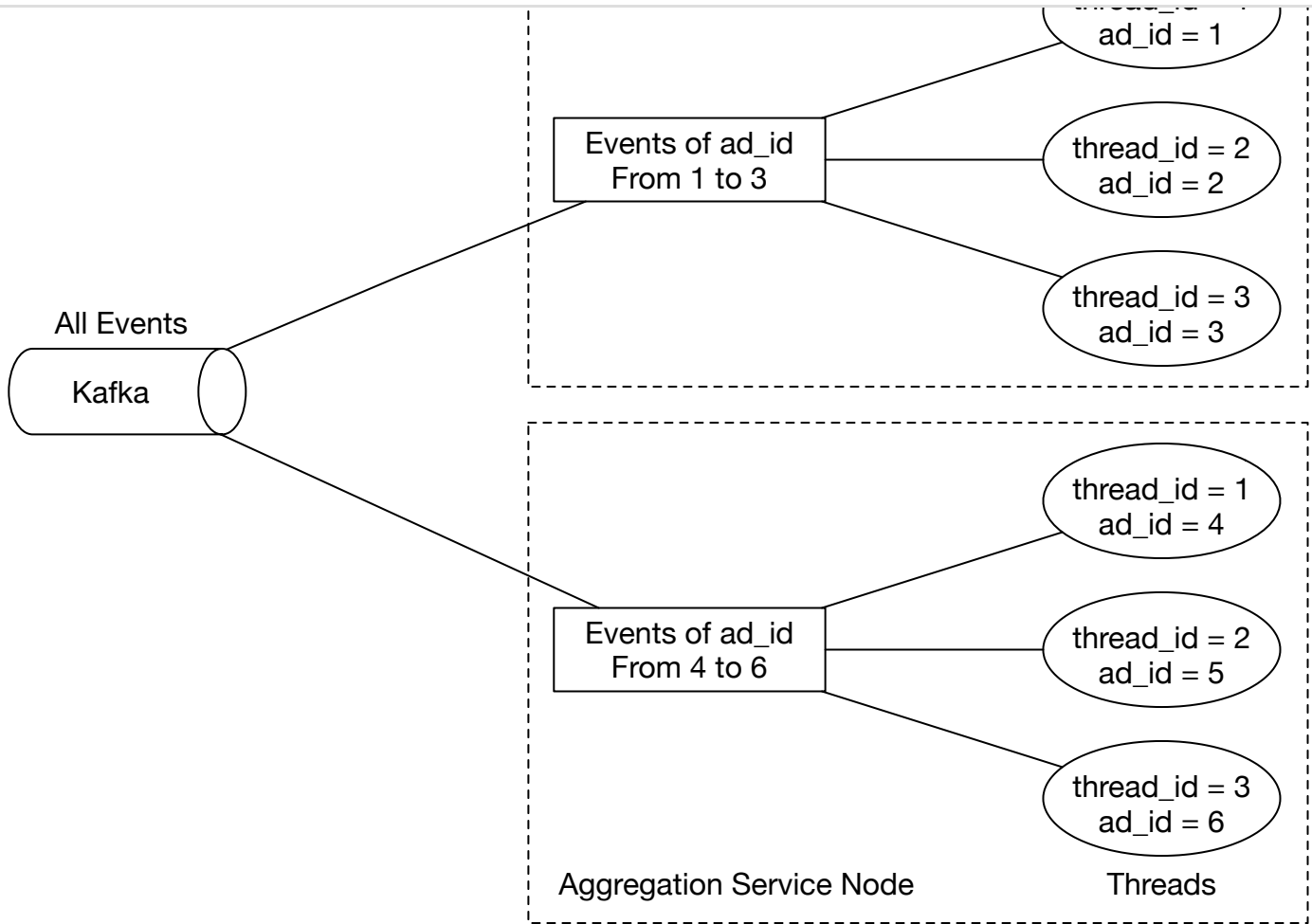
Figure 23 Multi-threading
