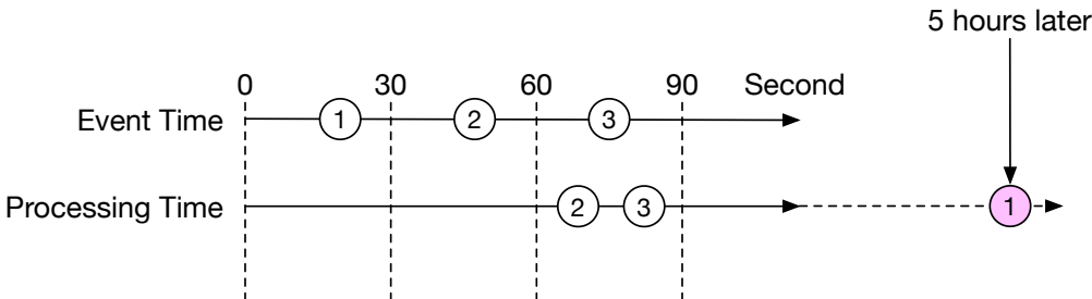
Figure 12 Late events
