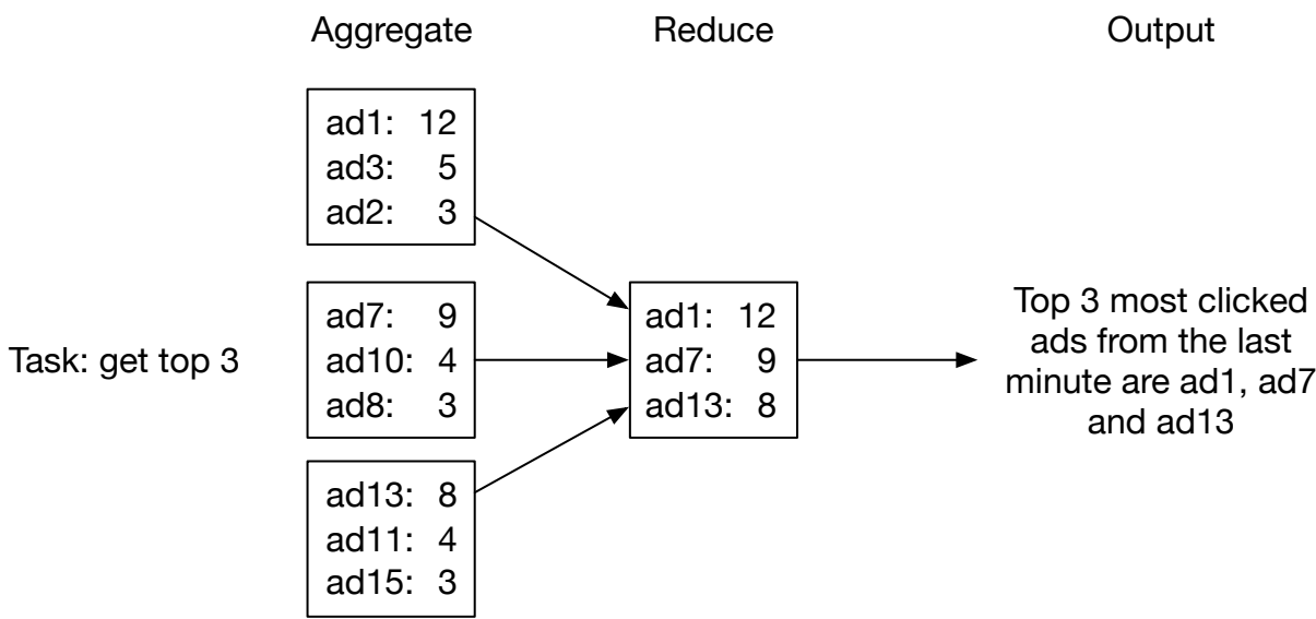
Figure 7 Reduce node
