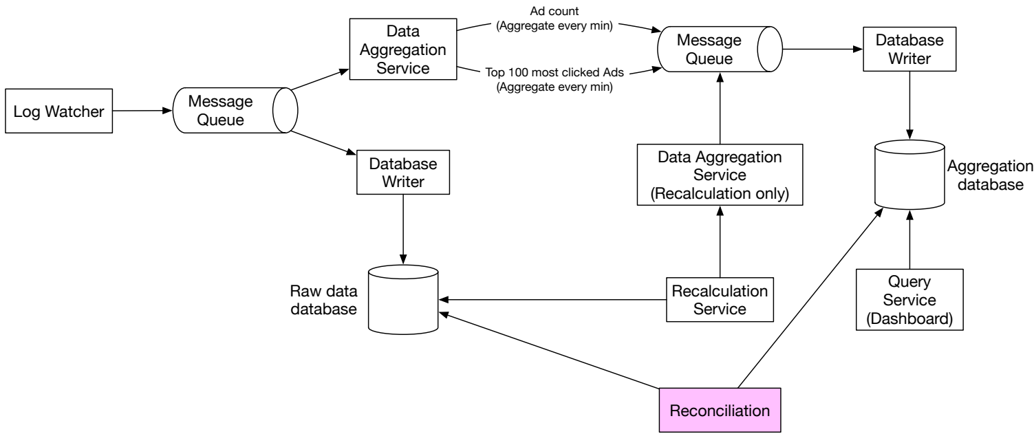
Figure 28 Final design
