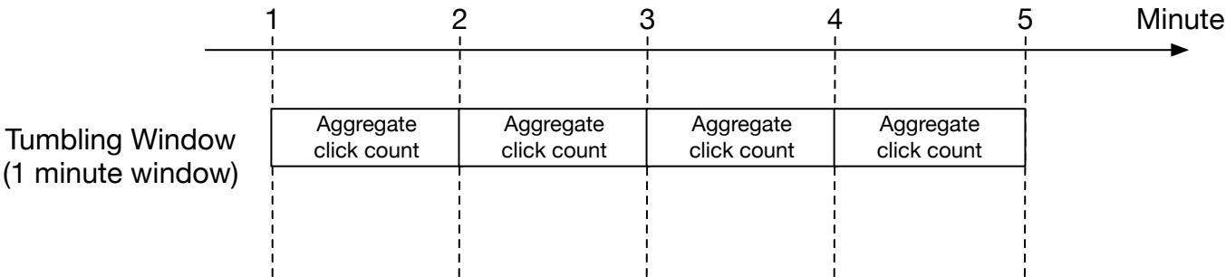
Figure 15 Tumbling window
