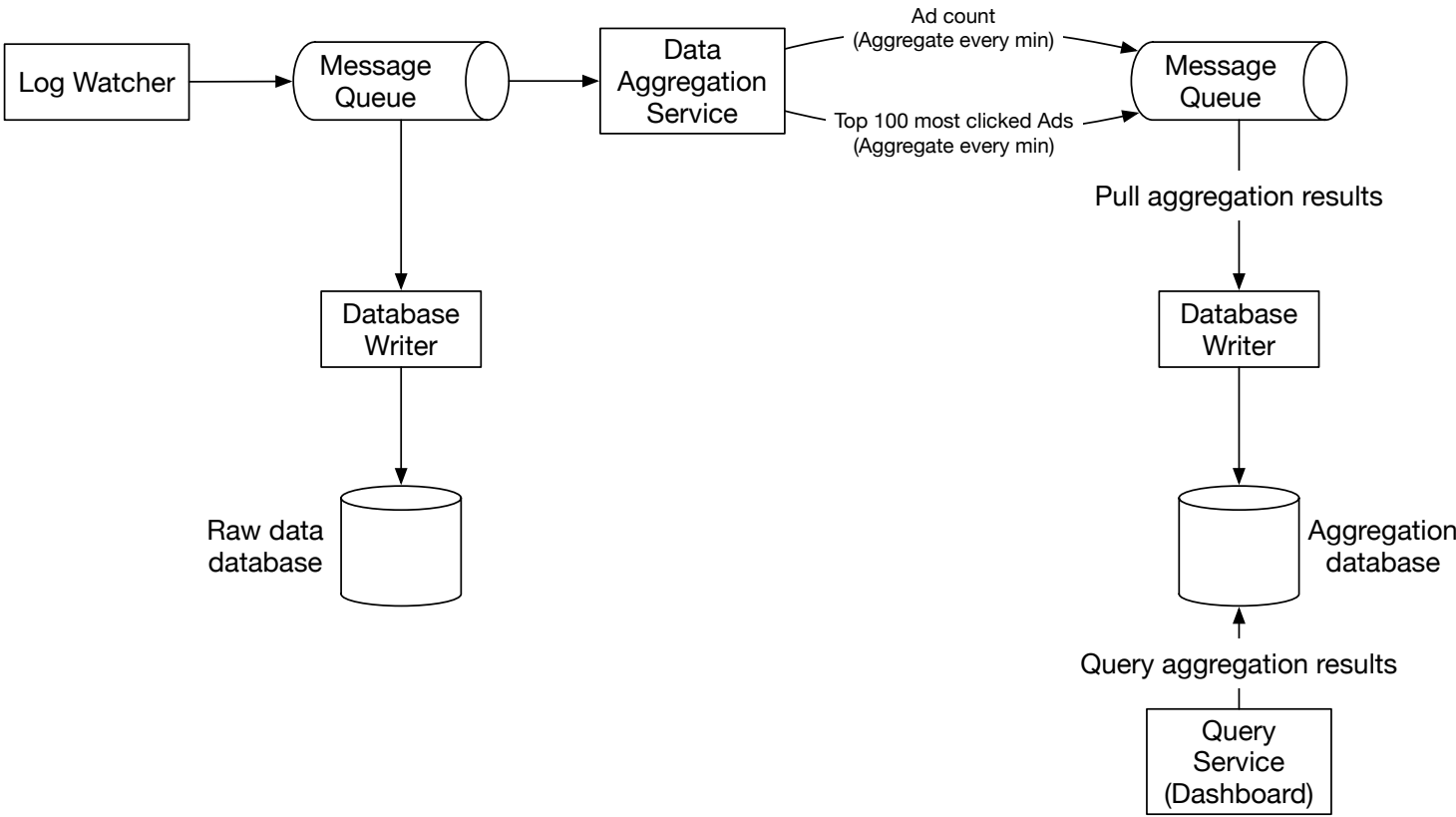
Figure 3 High-level design
